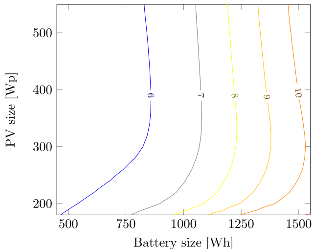
Fig. 9. Lifetime contours based on PV and (VRLA) battery sizes for a tier 3 load profile.
