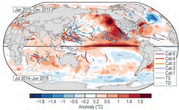
FIG. 4.18. Global summary of TC tracks with respect to SST anomalies for the 2015 TC season.
