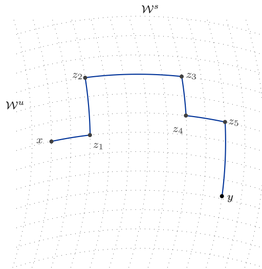
Figure 3.1: su-path
