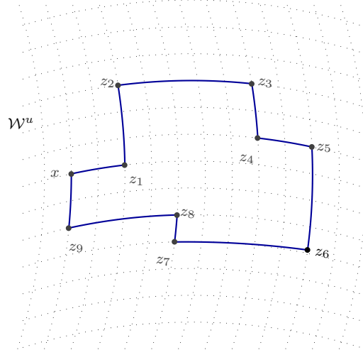
Figure 3.1: su-path
